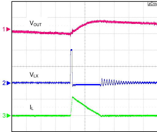
PFM Switching Waveform
